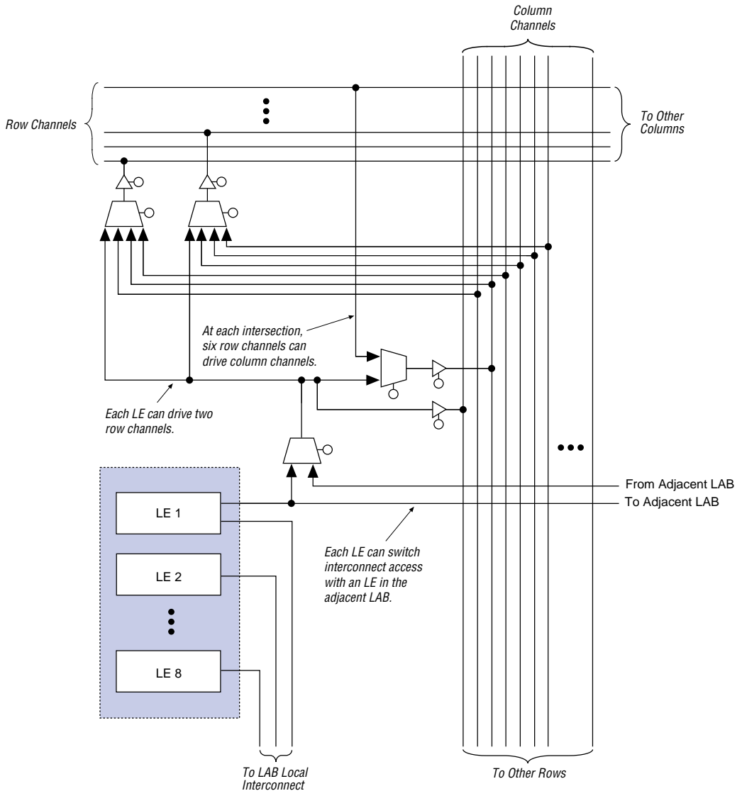
Figure 13. FLEX 10KE LAB Connections to Row &amp; Column Interconnect
