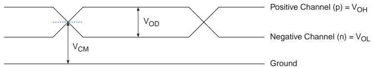
Single-Ended Waveform
