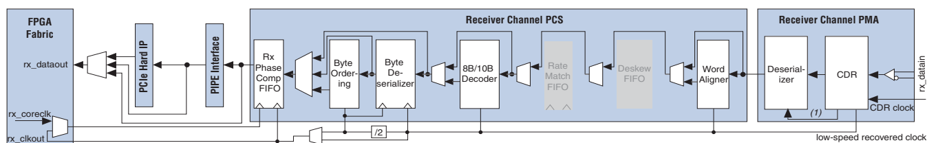
Figure 1–34. Receiver Only Datapath Clocking without Rate Match FIFO in Non-Bonded Channel Configuration
