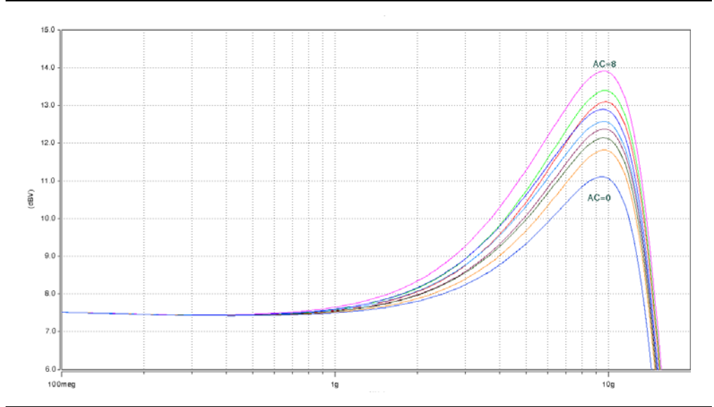
Figure 5. AC Gain Curves for GT Channels
