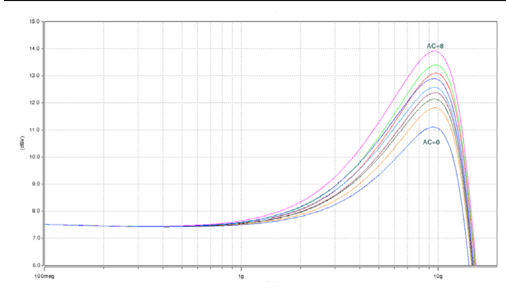
Figure 5. AC Gain Curves for GT Channels
