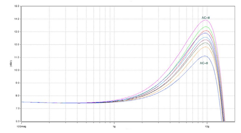
Figure 5. AC Gain Curves for GT Channels
